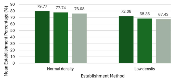
Figure 6.4: Effect of establishment method on variety establishment.
