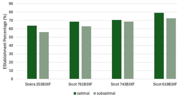
Figure 2.5: Effect of variety and field conditions on establishment percentage.
