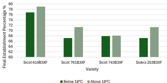
Figure 6.2: Effect of planting time and associated soil temperature conditions on establishment percentage for all CSD trials in 2023/24 season.
