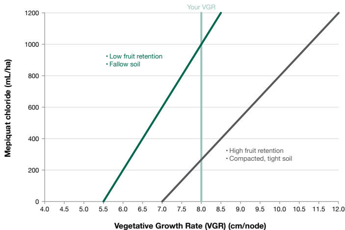
Figure 7.4: The VGR tool incorporating VGR measurements and other crop factors, to assess potential Mepiquat chloride use and rates (based on the older 38 g/l formulation)
