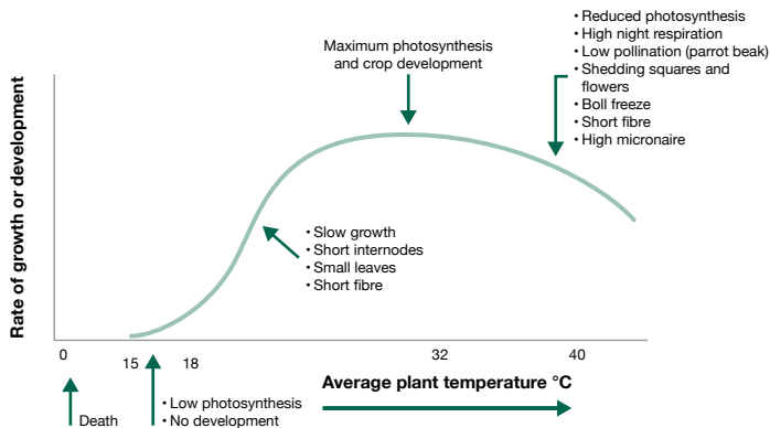
Figure 1.1: The effect of temperature stress on the physiological processes of the cotton plant, based on plant temperatures, not air temperatures. (Adapted from Bange and Brodrick, CSIRO, 2004).
